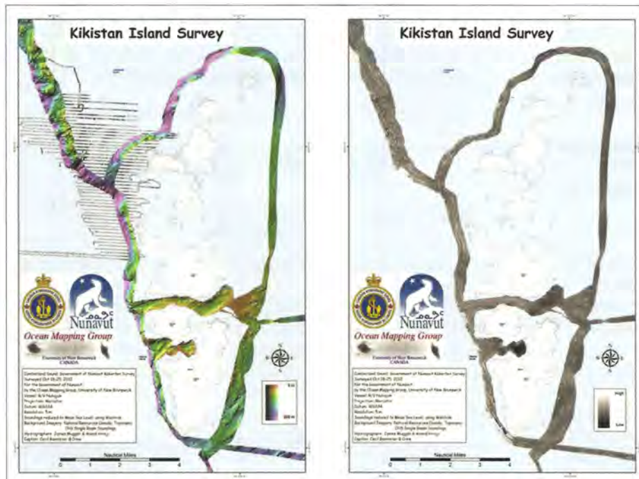
Figure 14: Nuliajuk multibeam access corridors around Kikistan Island Group. Left: bathymetry, Right: backscatter.
