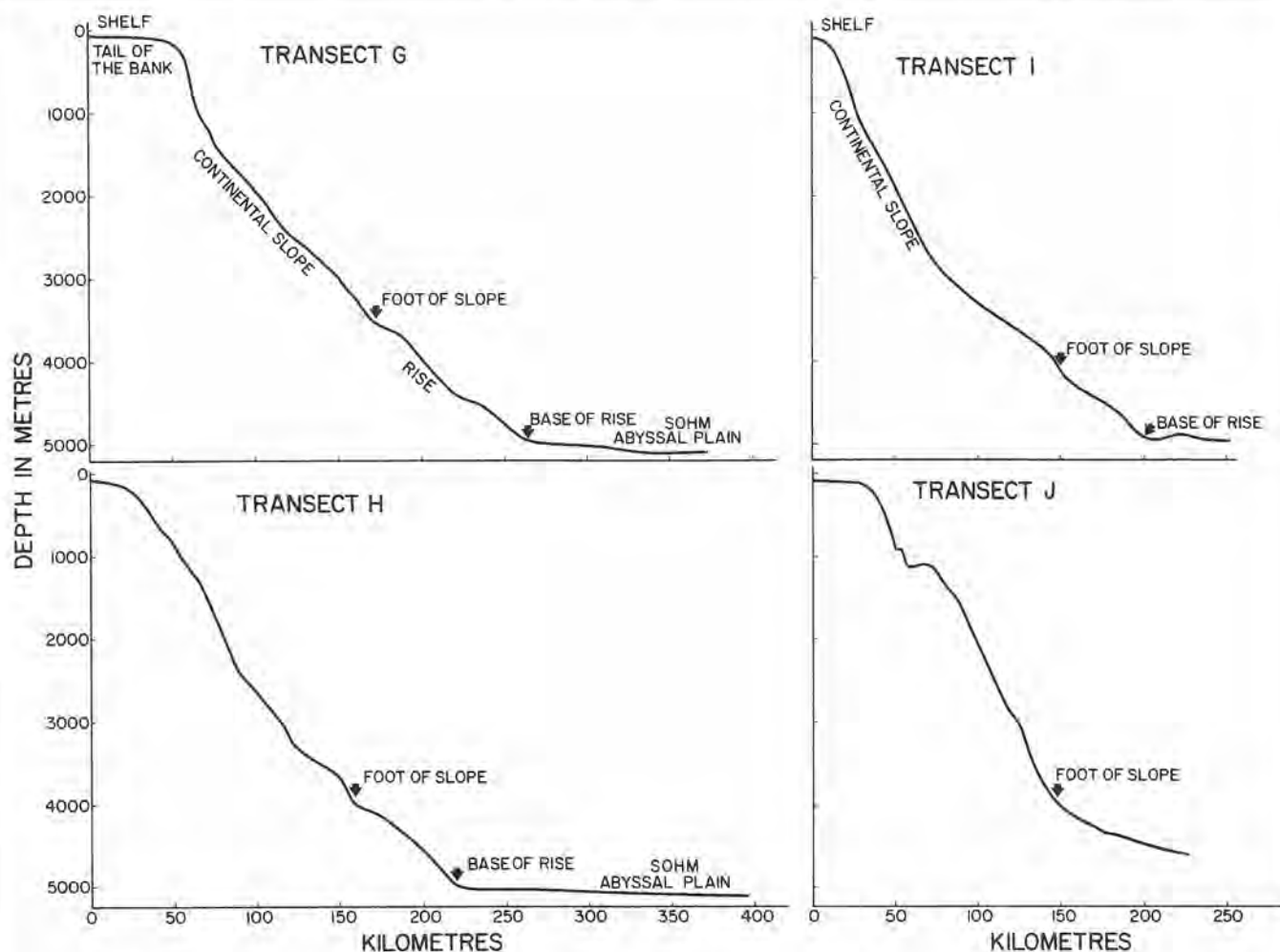
Figure 6: Bathymetric Profiles G, H, I, and J Showing Foot of the Continental Slope
