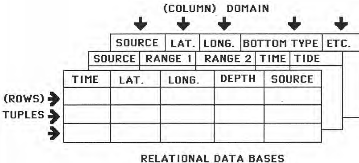
Figure 2: Classical Data Base Models
