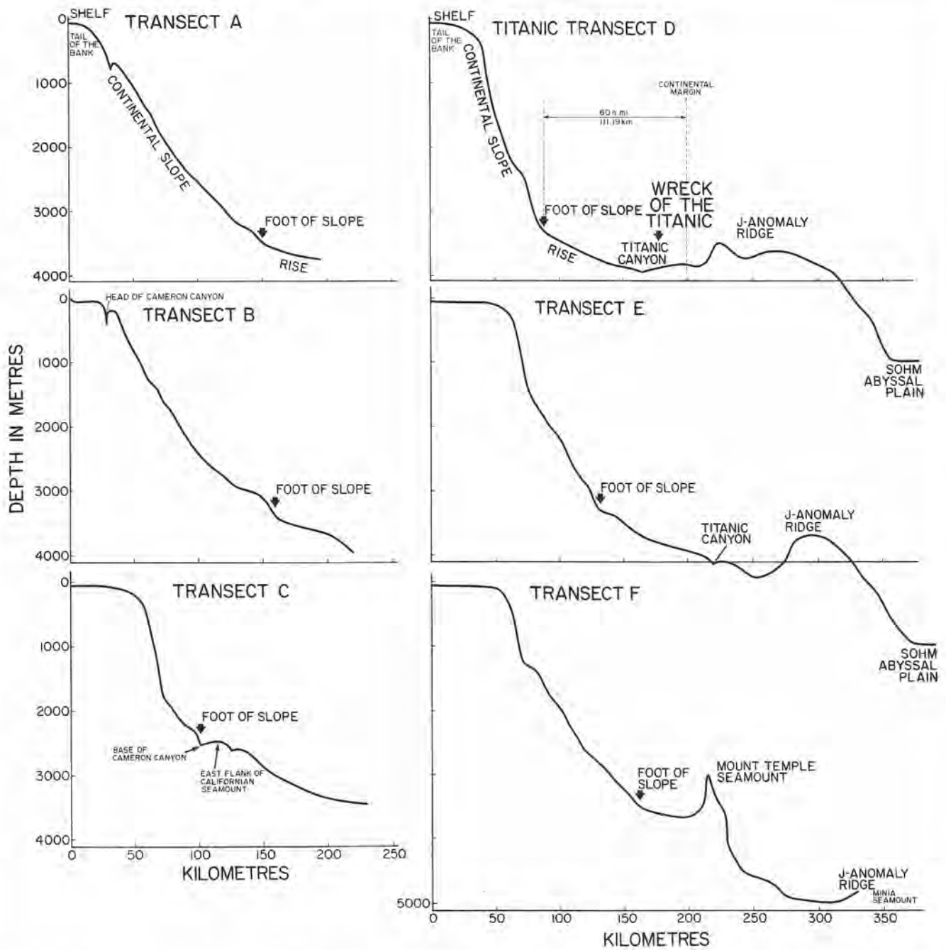
Figure 5: Bathymetric Profiles A, B, C, D, E and F Showing Foot of the Continental Slope
