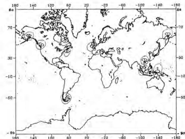
Figure 1: Locations of the largest tides in the world (1) Cap Astronomicheski (2) River Digoel (3) Pak-hoi (4) Muntok (5) Whaletown Bay (6) Cobequid Bay (7) Leaf Basin (8) Breachley Pier (9) Santa Craig (10) Anchorage
