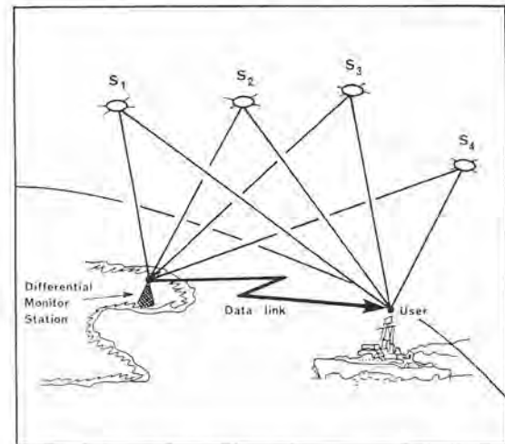
Figure 12. Differential GPS navigation concept. Variations in GPS ranges or coordinates are measured by monitor and sent to users over data link, to correct their positions.
